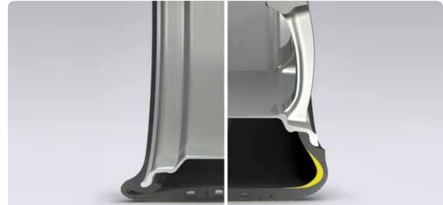
Tyre with Run-Flat Technology
